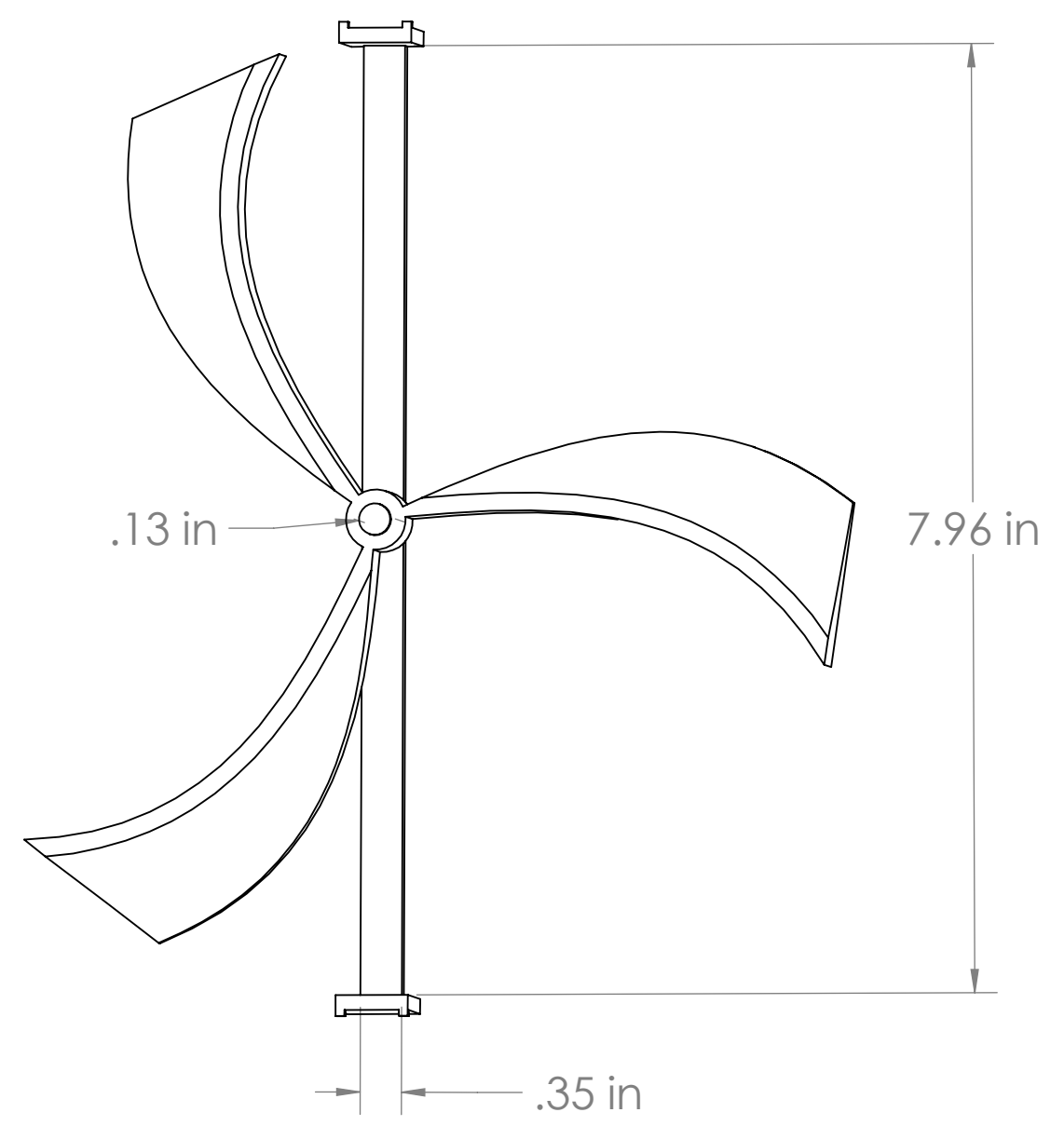
FRONT VIEW
